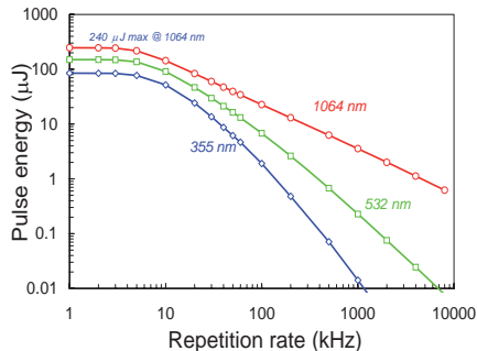
Typical pulse energy versus repetition rate for 1064 nm, 352 nm, and 355 nm
