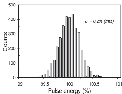
Pulse energy stability. The histogram shows the energy distribution of 3500 pulses with an rms fluctuation of 0.2%
