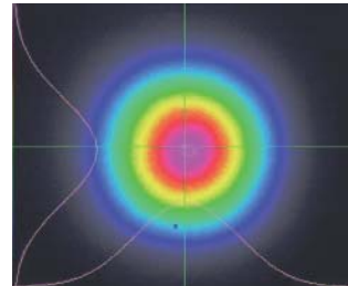
Output beam profile
