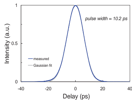
Autocorrelation trace
